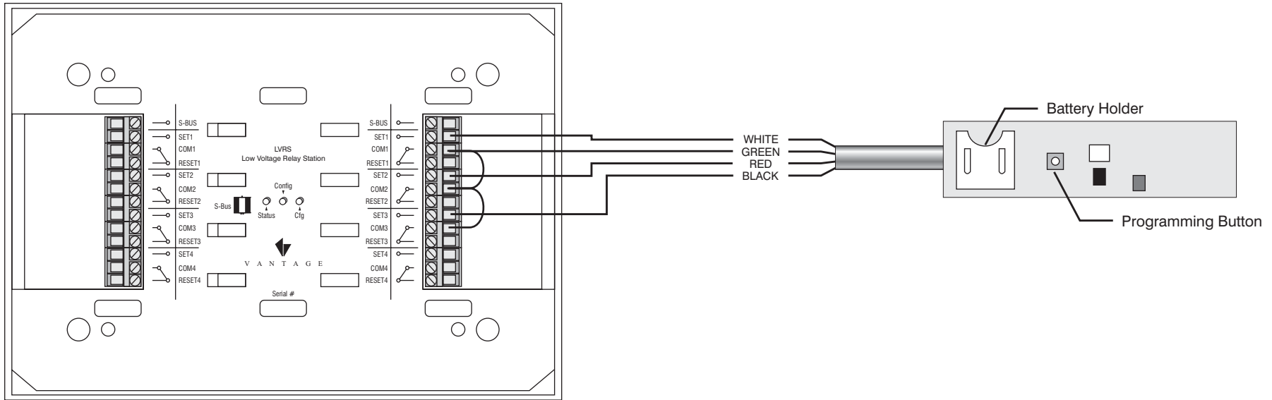
Vantage - Low Voltage Relay System (LVRS)
